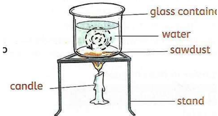
Fig. 4 Convection currents in liquids
